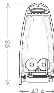
2 batterie da 3,6V incluse 2 3,6V batteries included
