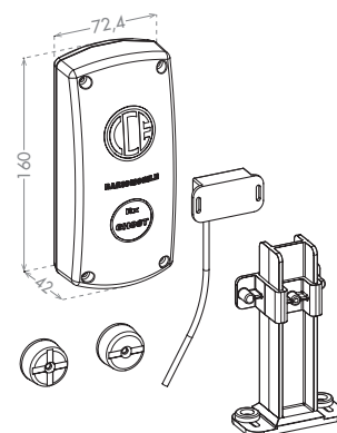
2 batterie da 3,6V incluse 2 3,6V batteries included
